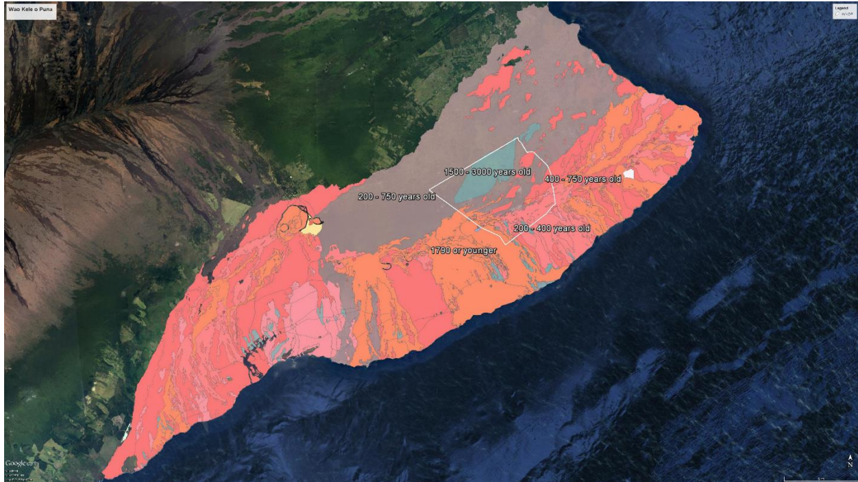
The Brown marking notes the 'Ailā'au Flow – the Blue the Kīpuka and the white line outlines the Wao Kele o Puna Boundary
